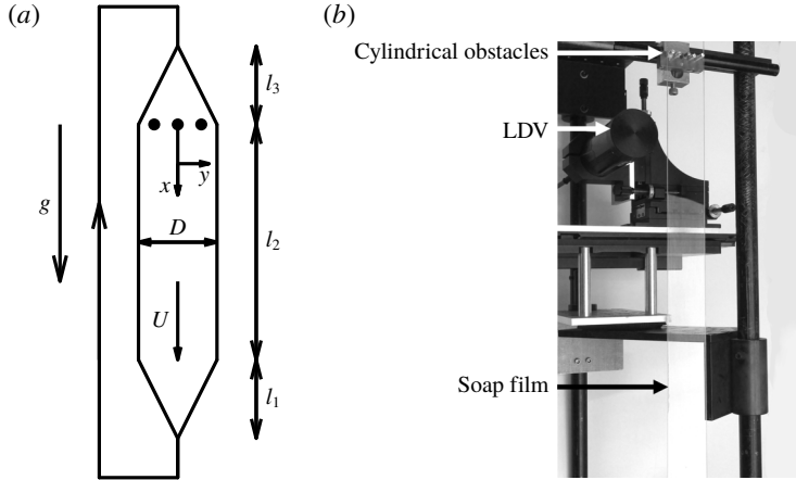
FIGURE 7. (a) Gravity g drives a 3 \mu\text{m} thick soap film with a velocity of around U = 2 \text{ m s}^{-1} between two wires, that form a vertical channel, with a diverging width, a constant width D = 0.06 \text{ m} and a converging width. The lengths of the respective sections are l_3 = 0.7 \text{ m} , l_2 = 1 \text{ m} and l_1 = 0.45 \text{ m} . Soap is collected at the channel exit, pumped upwards and injected at the channel entrance. Three cylinders are placed in the film to generate 2-D turbulence. The downstream distance to the cylinders and the wall normal distance to the channel centreline are denoted x and y , respectively. (b) Photograph of the set-up, showing the cylindrical obstacles, the LDV probe and the soap film.
