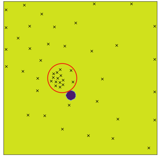
Figure 2: A swarm with a memory length of t_{\text{mem}} = 20 tracking an evasive target. Agents clustering in the wrong location due to the exploitation of outdated information circled in red when using excessive memory lengths.
