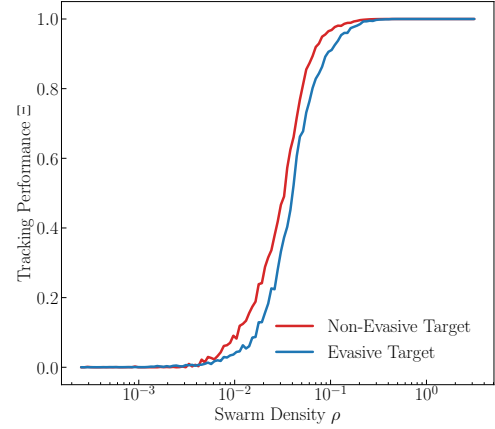
Figure 5: The effect of a target's movement policy on a tracking swarm's performance at different densities.
